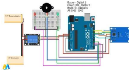
Figure 5. Smart Doorlock Hardware Design
