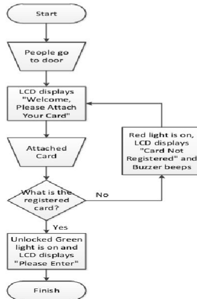
Figure 11. Flowchart of Smart Doorlock System
