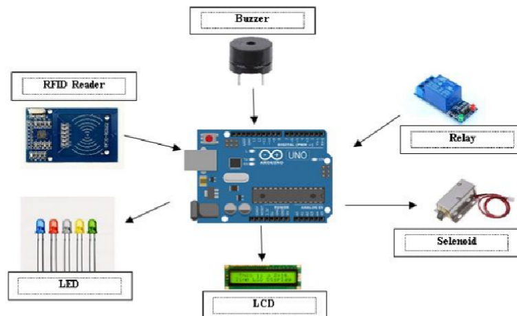
Figure 4. Flow System
