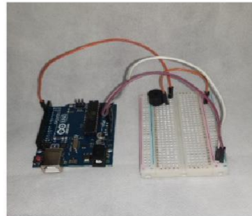
Figure 17. Buzzer Installation
