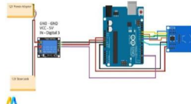
Figure 6. Design of Solenoid Doorlock and Relay Module
