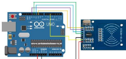
Figure 9. Desain RFID
