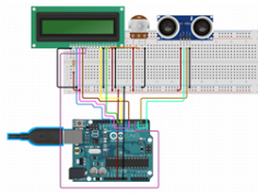
Figure 10. Body Height Measuring Tool Design
