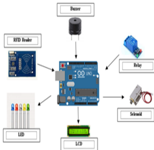
Figure 4. Flow System
