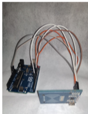
Figure 13. RFID Installation
