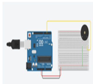
Figure 10. Desain Buzzer
