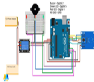
Figure 5. Smart Doorlock Hardware Design
