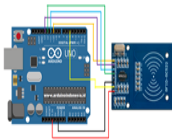
Figure 9. Desain RFID
